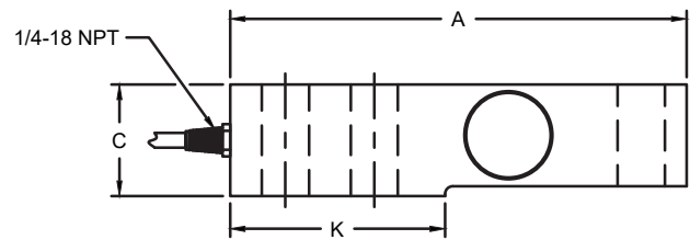
CG-23-SSW-1 NON-THREADED LOAD HOLE
