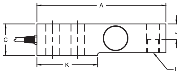
CG-23-SSW THREADED LOAD HOLE
