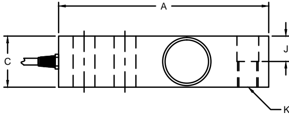
CG-23 THREADED LOAD HOLE
